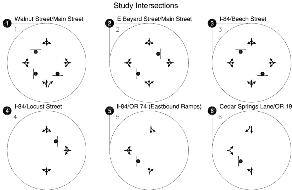
Exhibit 3. Study Intersection Traffic Control and Lane Configurations
